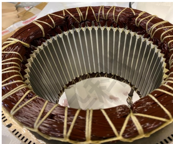
Figure 3: Stator Assembly
